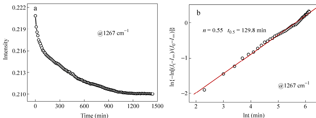
Fig. 8 (a) Intensity change of PLLA at 1267 cm -1 and (b) the curve fitting results on the growth of mesophase using the intensity change at 1267 cm -1 during the aging process
