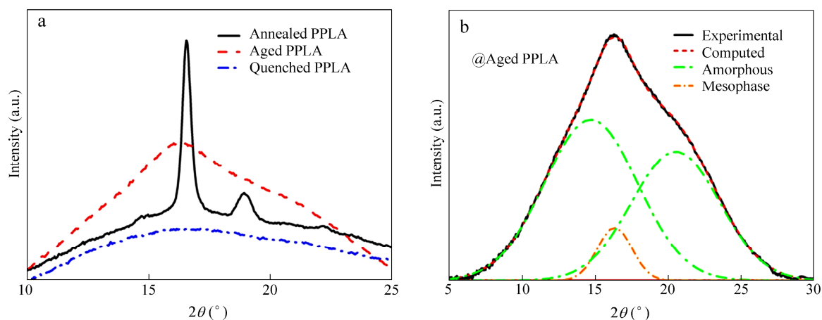
Fig. 2 (a) Azimuth-integrated WAXD intensity profile of quenched and aged PPLA (1D-WAXD profile of PPLA annealed at 120 °C for 1 h is also presented for comparison), and (b) the curve fitting analysis of the WAXD intensity profile of aged PPLA
