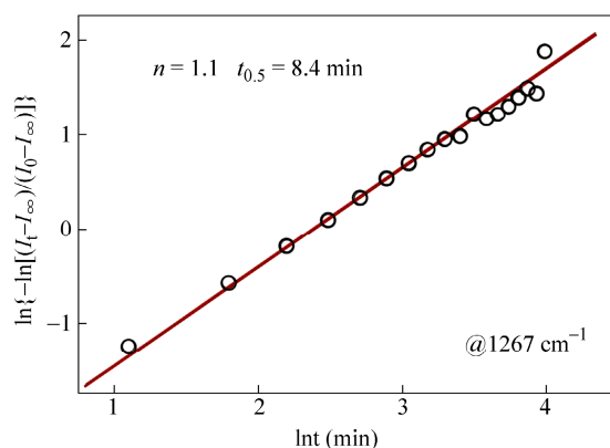
Fig. 7 Curve fitting results on the growth of mesophase of aged PPLA using the intensity change at 1267 cm -1 during the aging process at 53 °C for 1 h
